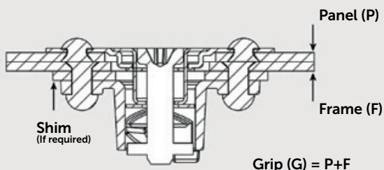
SHIM 0.8MM 205-9008
