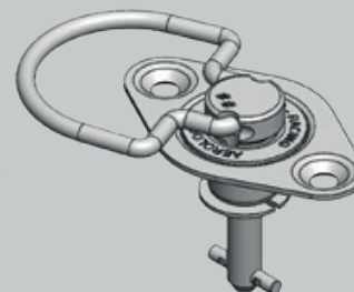
BAIL HANDLE COUNTERSUNK FIXING HOLES (1MM MIN PANEL THICKNESS) 200-5100 SERIES
